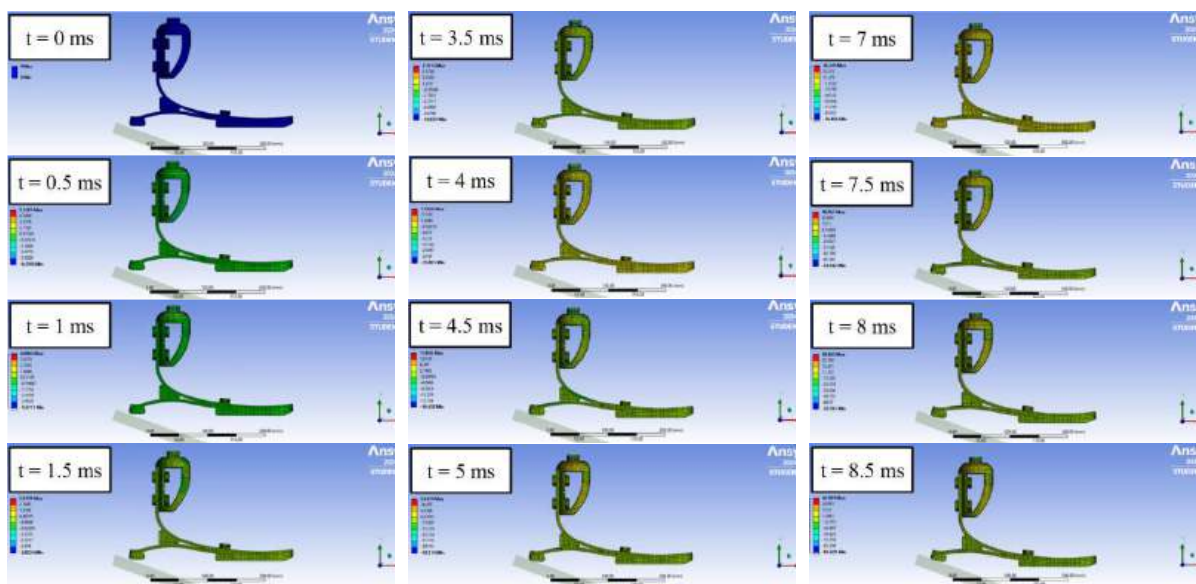
Appendix I FEA explicit dynamic models of foot flat gait
