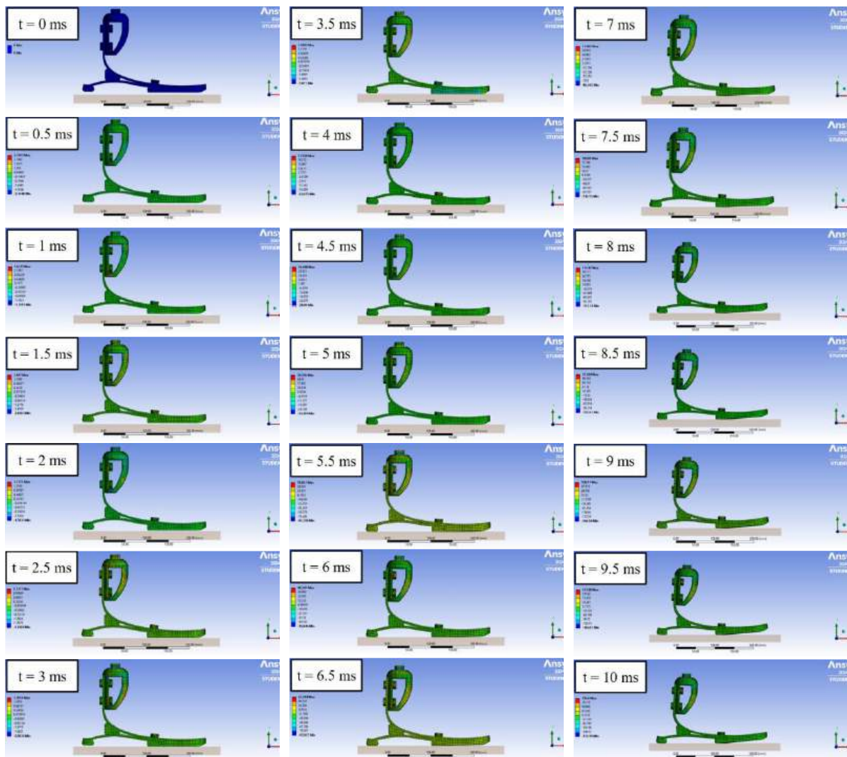
Appendix I FEA explicit dynamic models of foot flat gait
