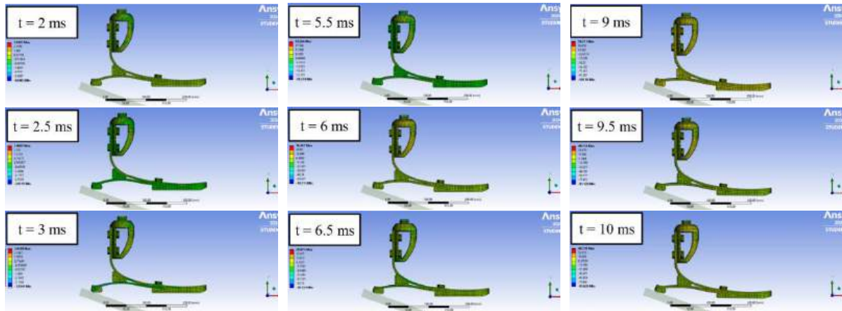
Appendix II FEA explicit dynamic models of heel strike gait
