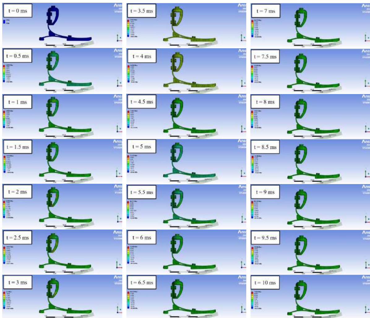
Appendix III FEA explicit dynamic models of toe strike gait
