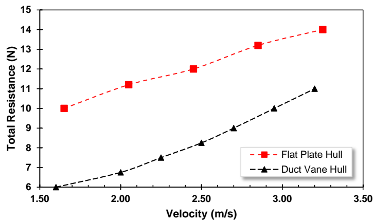
Figure 8 Comparison of the total resistance of the application of the duct vane
