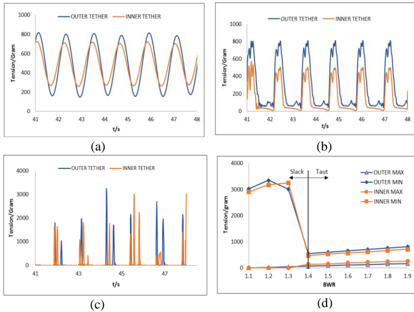
Figure 7 Time series of SFT tether tension force; (a) BWR=1.9; (b) BWR=1.4; (c) BWR =1.3;(d) maximum and minimum tether tension force (individual wave)
