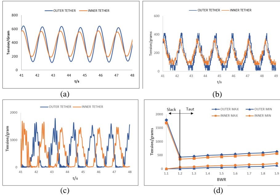
Figure 6 Time series of SFT tether tension force: (a) BWR = 1.9; (b) BWR = 1.2; (c) BWR = 1.1; (d) maximum and minimum tether tension force (significant wave)
