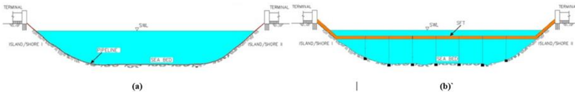
Figure 1 (a) Conventional pipeline case-1; (b) proposed pipeline using SFT case-1
