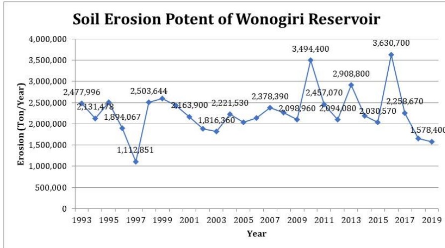
Figure 5 Soil erosion prediction in year 1993 – 2019
