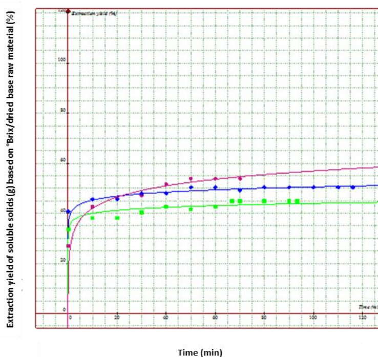
Figure 5 Overall extraction yield curve of upscaling
