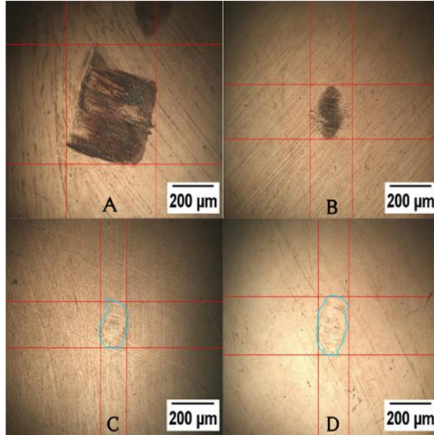
Figure 9. The HFR test results also show the WSD on the steel ball surfaces after lubrication with: (A) pure PAO oil, (B) GO 1wt%-PAO, (C) GO 3wt%-PAO, and (D) GO 3wt%-PAO. The images illustrate the progressive reduction in wear scar size with increasing GO content, indicating enhanced antiwear performance due to the formation of protective tribofilm facilitated by GO additives.
