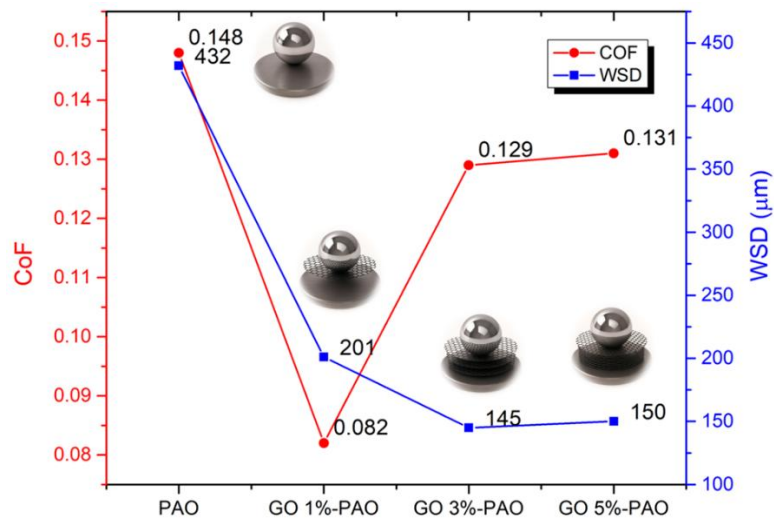
Figure 10. Comparison of the CoF and WSD values for four lubricant samples: pure PAO, 1%, 3%, and 5% additives. The graph illustrates the tribological performance under identical test conditions.
