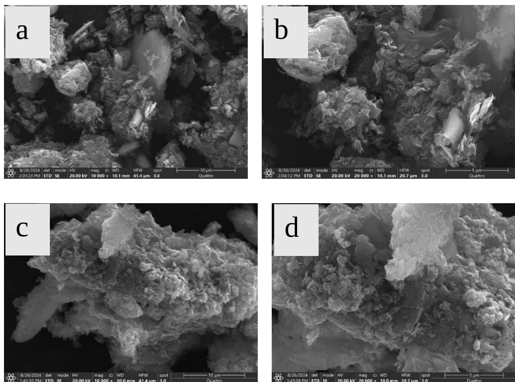
Figure The SEM characterisation results (a) rGO \times 10000 magnification, (b) rGO \times 20000 magnification, (c) CuNP-rGO-PANI \times 10000 magnification, (d) CuNP-rGO-PANI \times 20000 magnification
