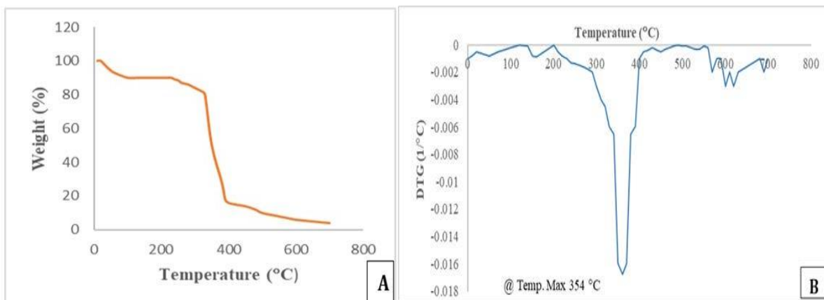
Figure 9 Thermogram (TG) of cellulose ester (A), derivative thermogram analysis (DTG) of cellulose ester (B).
