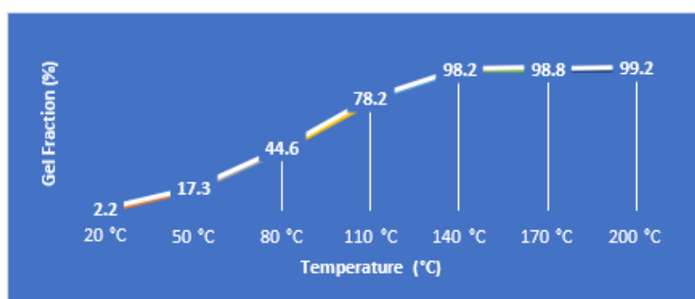
Figure 10 Gelation characteristics with increasing temperature
