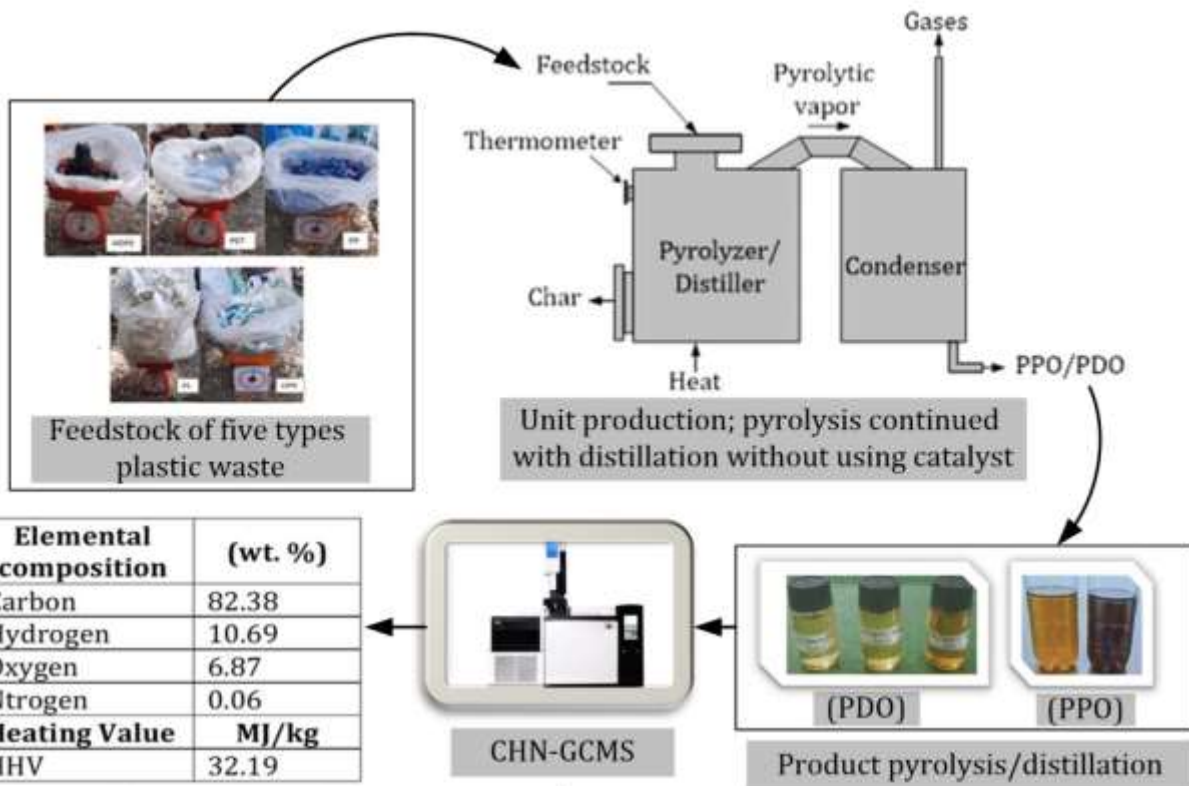
Elemental composition of PDO through CHN Method
