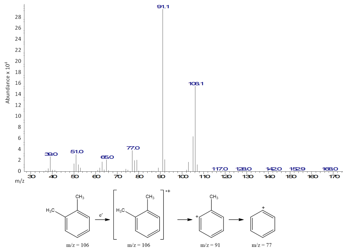
Figure S4. Mass spectroscopy of organic phase with xylene solvent (retention time = 2.7 minute)
