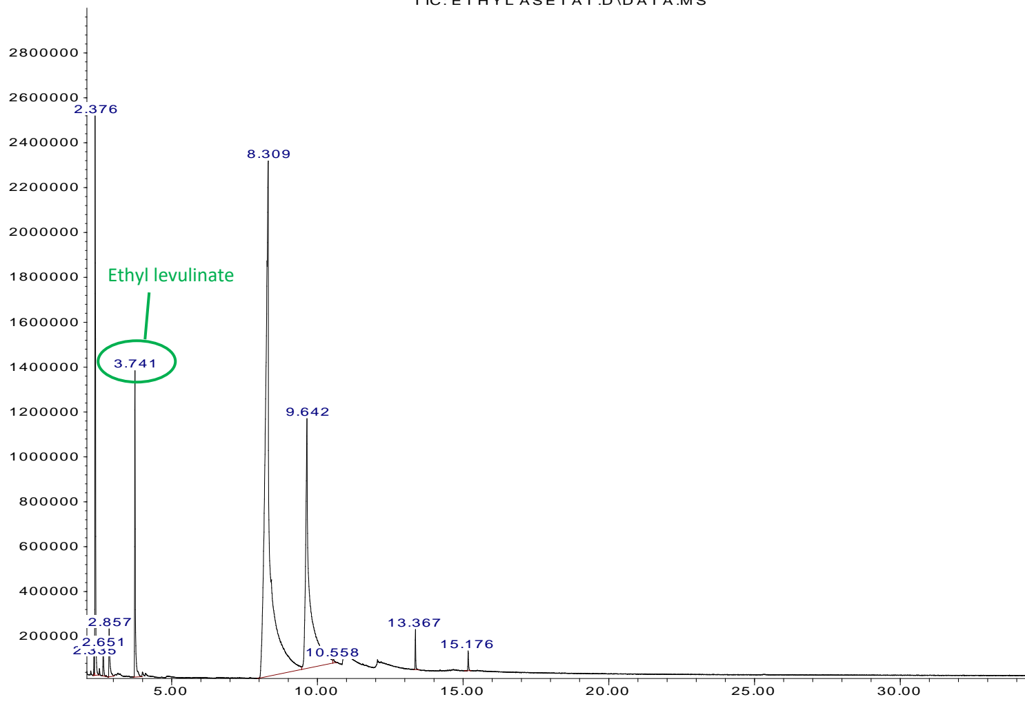
Figure S1. Chromatogram of the organic phase with ethyl acetate solvent
