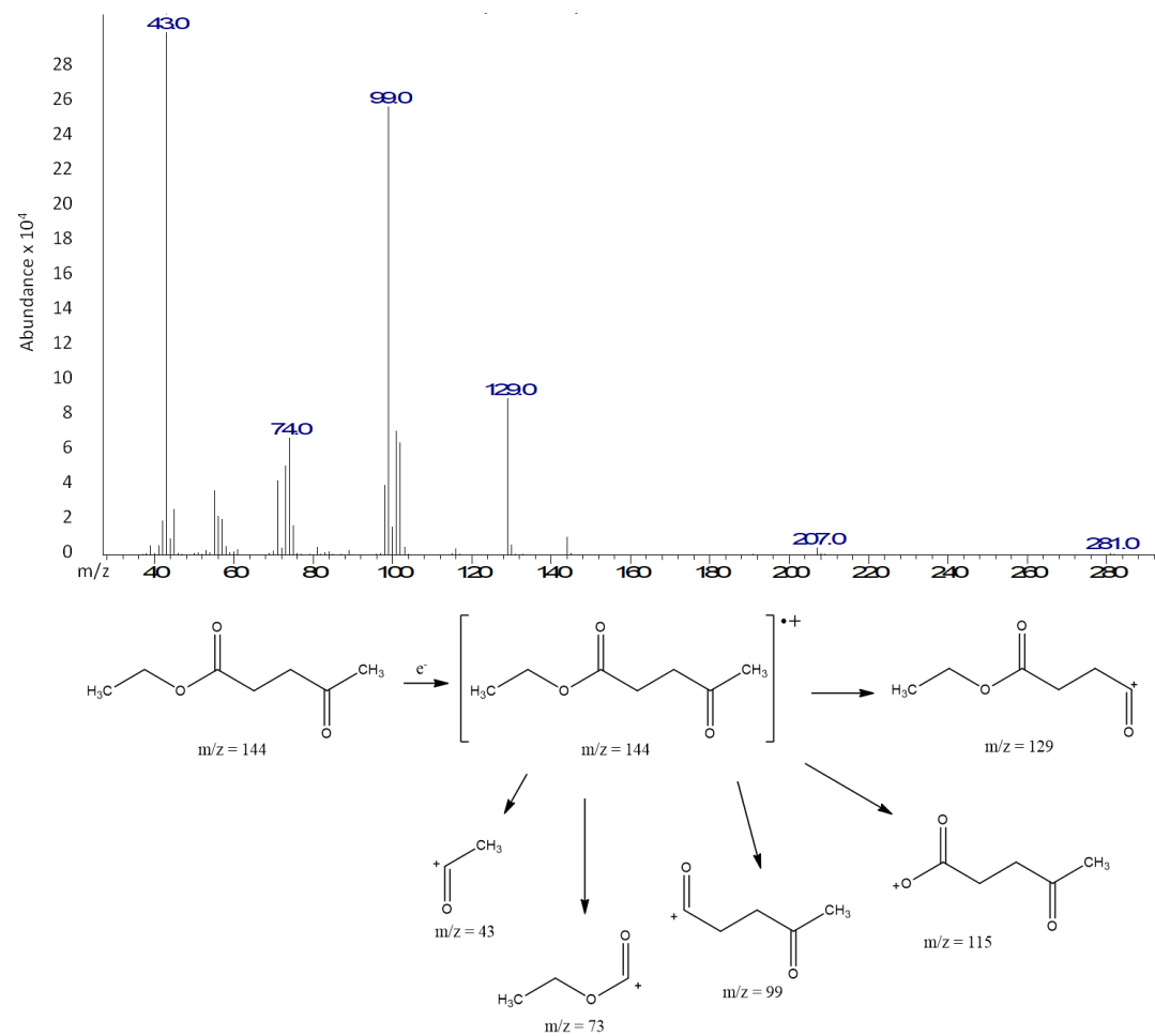
Figure S2. Mass spectroscopy of organic phase with ethyl acetate solvent (retention time = 3.7 minute)
