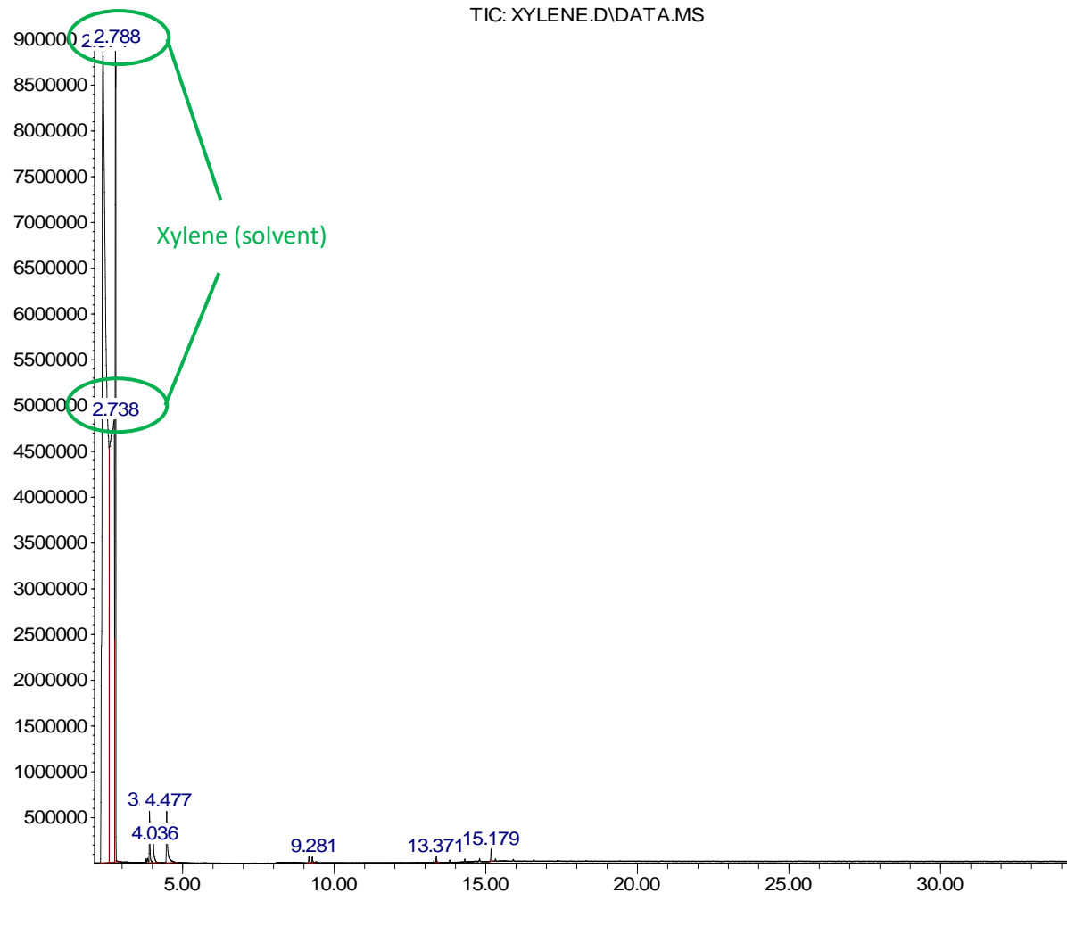
Figure S3. Chromatogram of organic phase with xylene solvent
